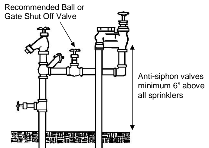
Hose Bib with Back Flow Device Installed
