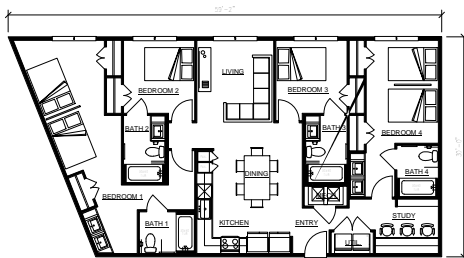
10 UNIT F3 1/8"=1'-0" 1595 SF
