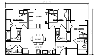
1 UNIT C1 1/8"=1'-0" 1043 SF
